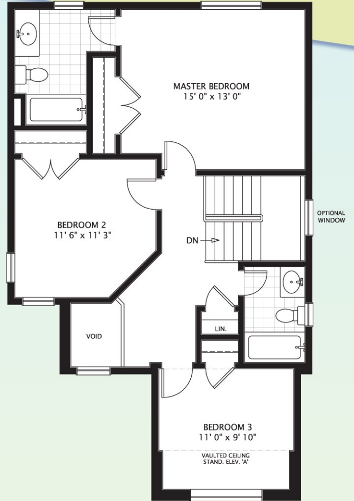
SECOND FLOOR - ELEV. A & B
