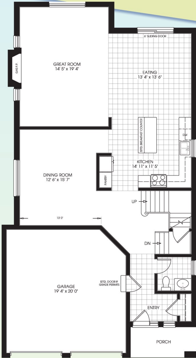
GROUND FLOOR - ELEV. A & B
