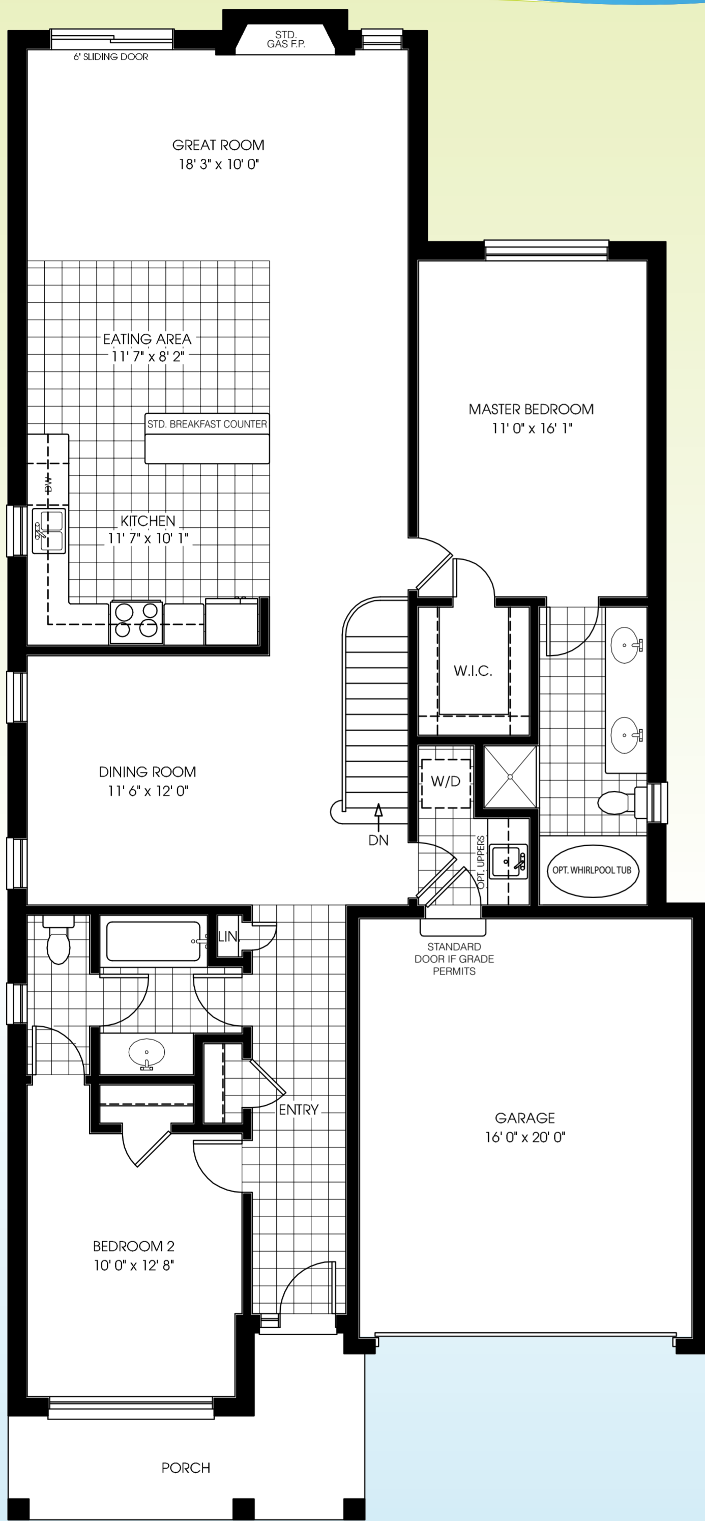
MAIN FLOOR - ELEV. A
