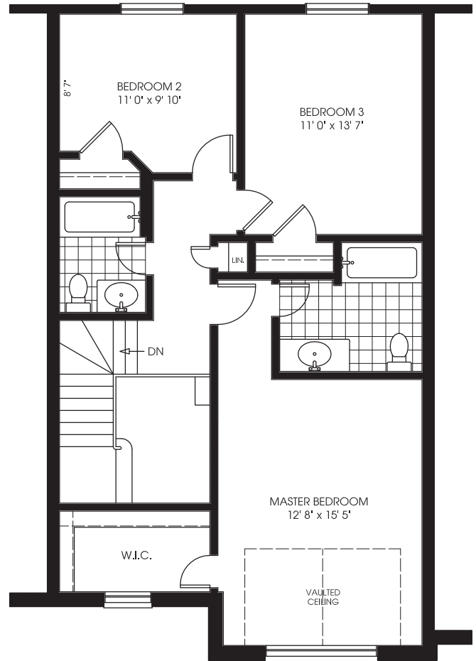
SECOND FLOOR
