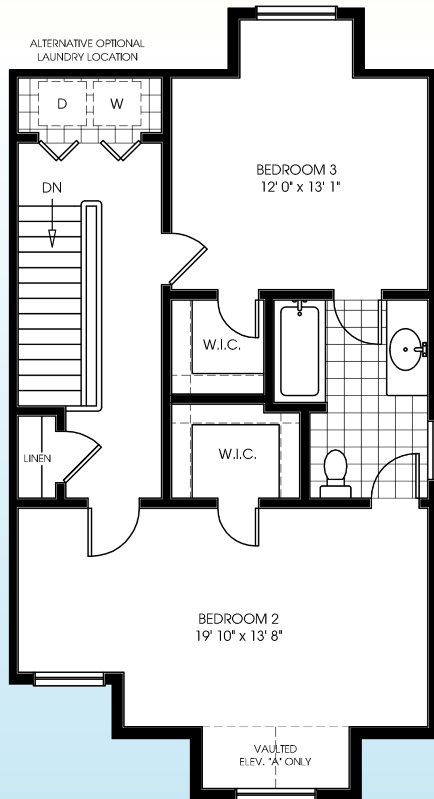
ALT. SECOND FLOOR - ELEV. A
