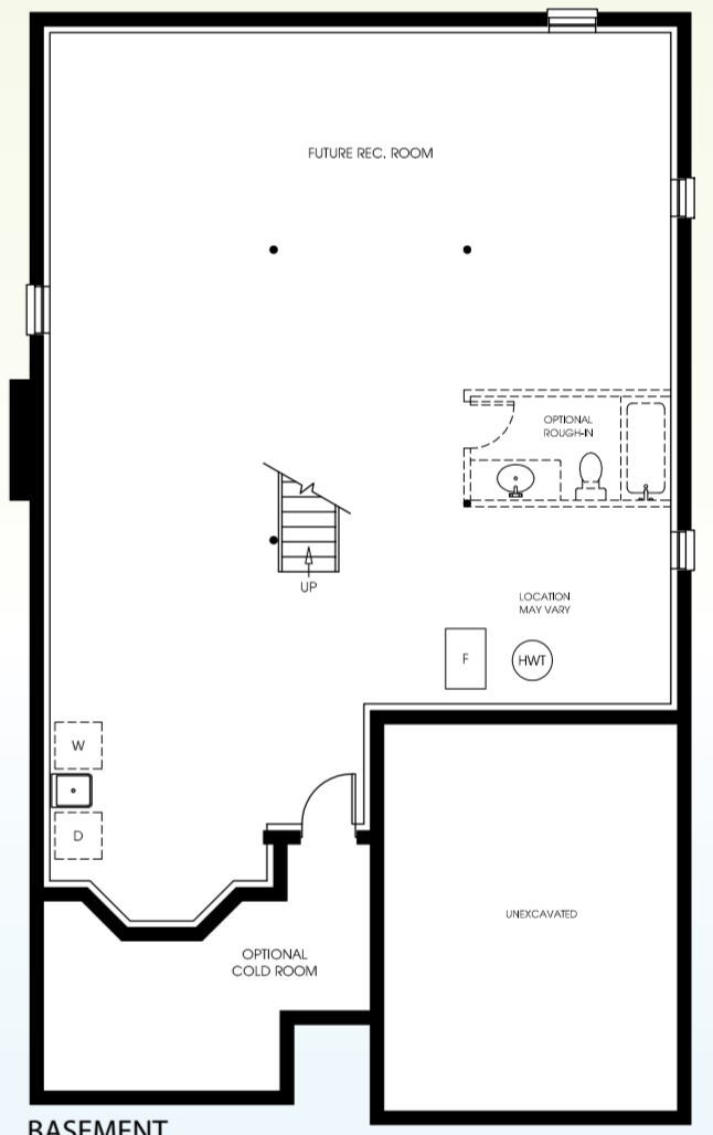
BASEMENT
