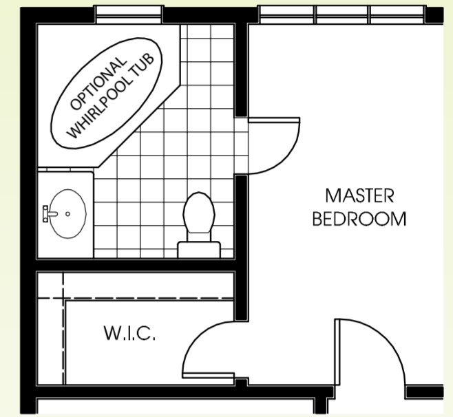
ALT. ENSUITE BATHROOM
