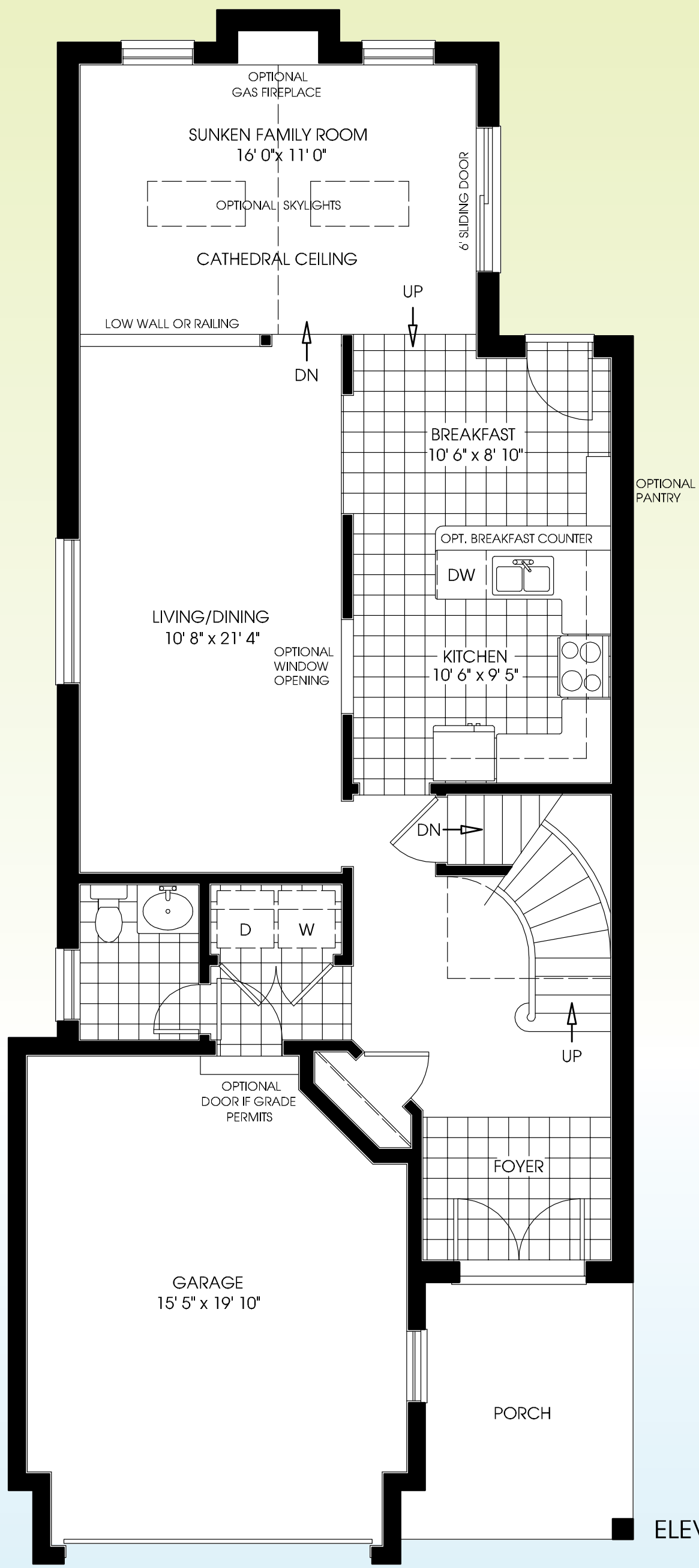
GROUND FLOOR
