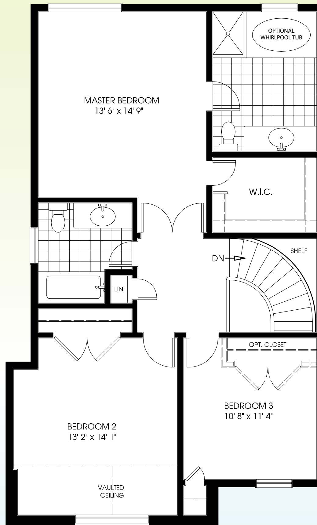
SECOND FLOOR - ELEV. A
