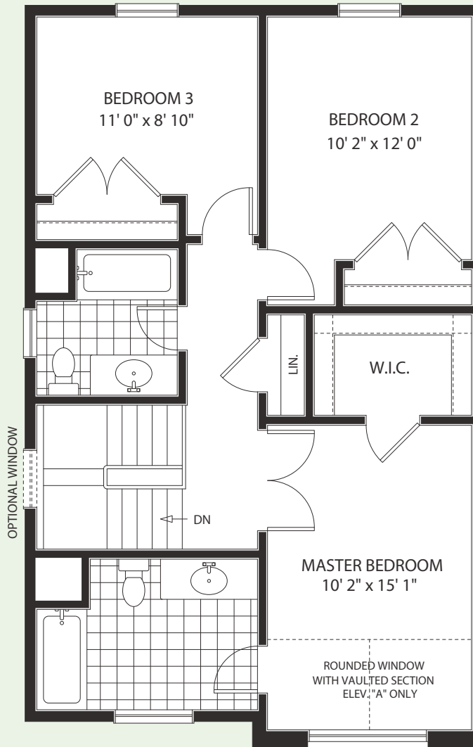
SECOND FLOOR - ELEV. A 1573 SQ.FT.
