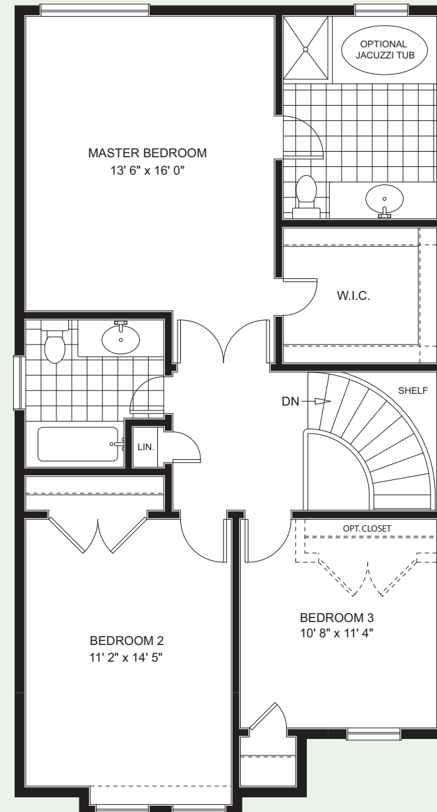
SECOND FLOOR ELEV. A - 1752 SQ.FT.
