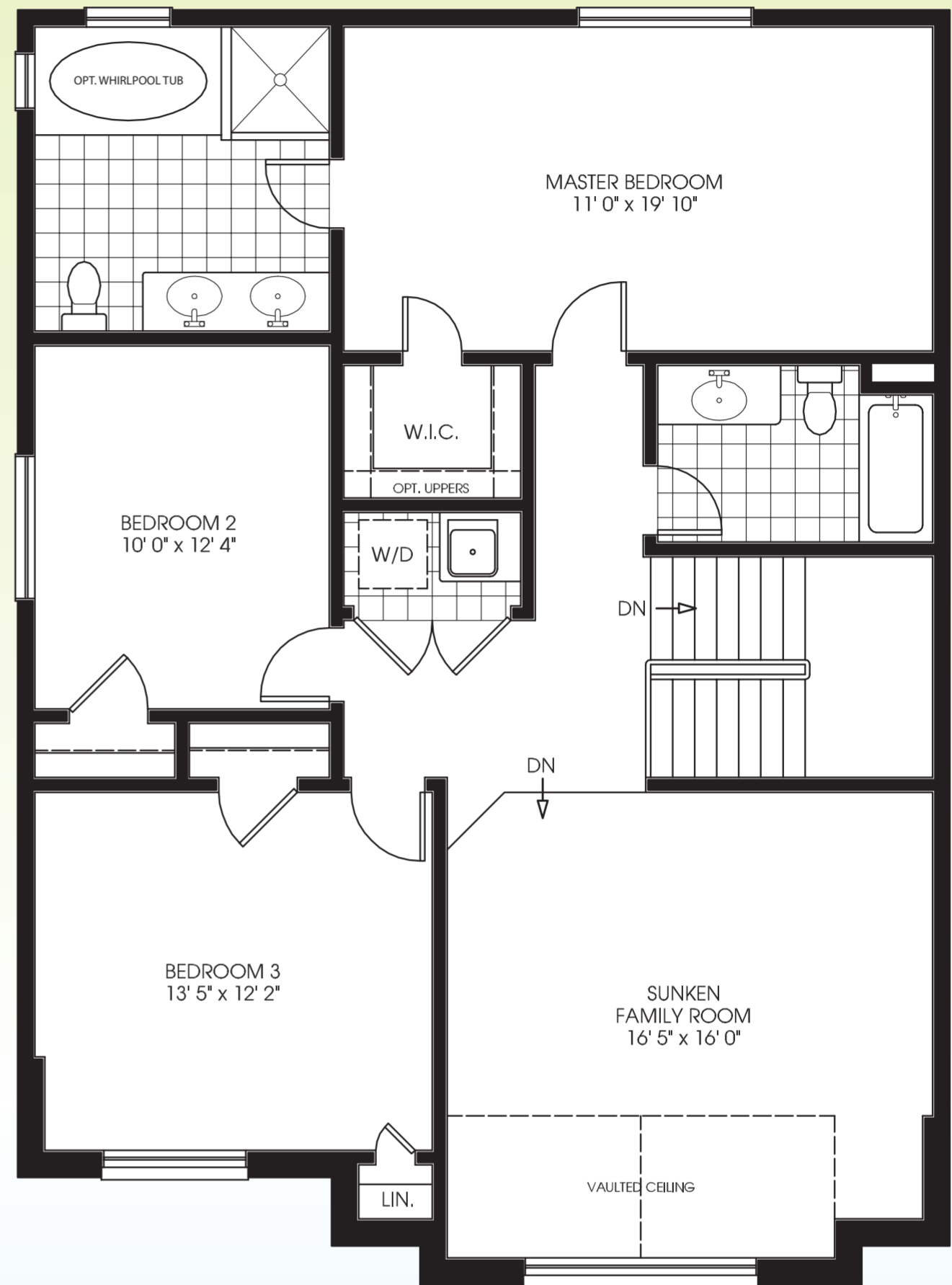
SECOND FLOOR - ELEV. A
