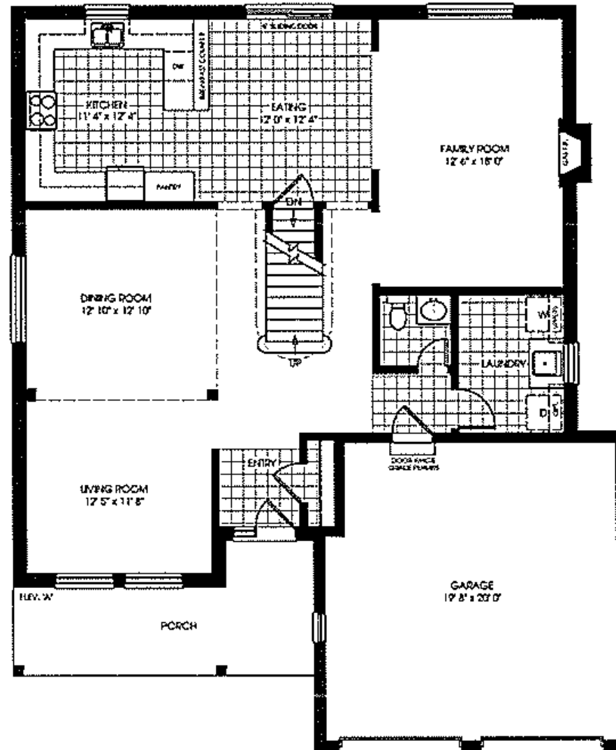
MAIN FLOOR
