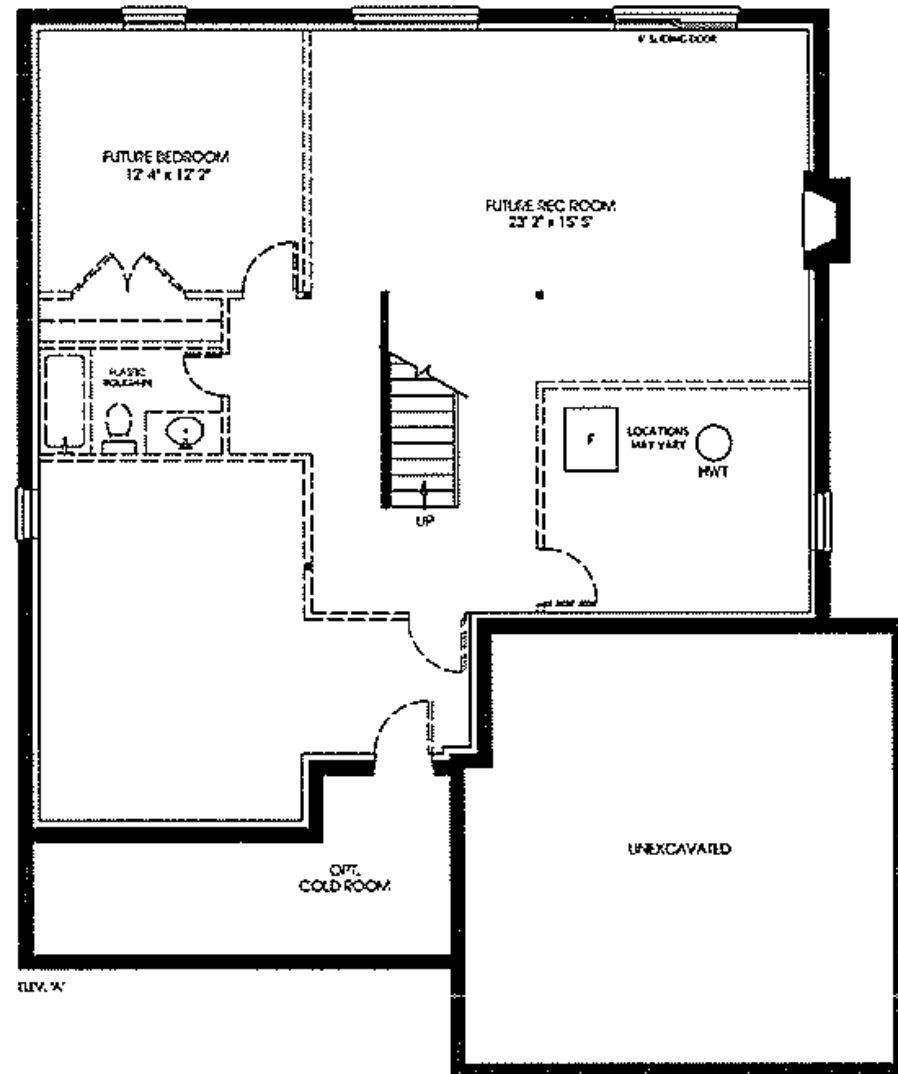
BASEMENT
